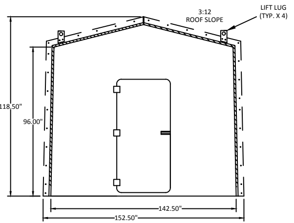
FRONT ELEV.
