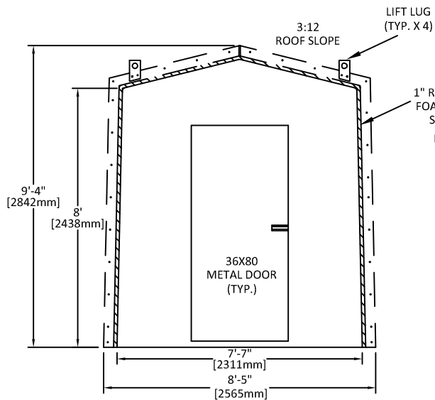
FRONT ELEV.
