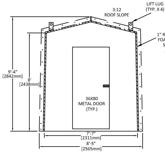
FRONT ELEV.
