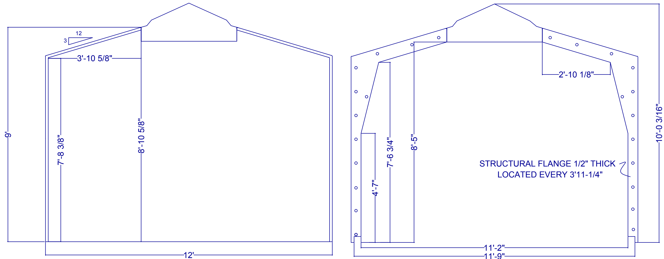
CROSS SECTION
