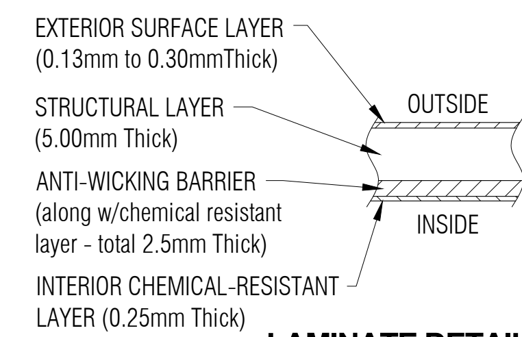
LAMINATE DETAIL E NTS
