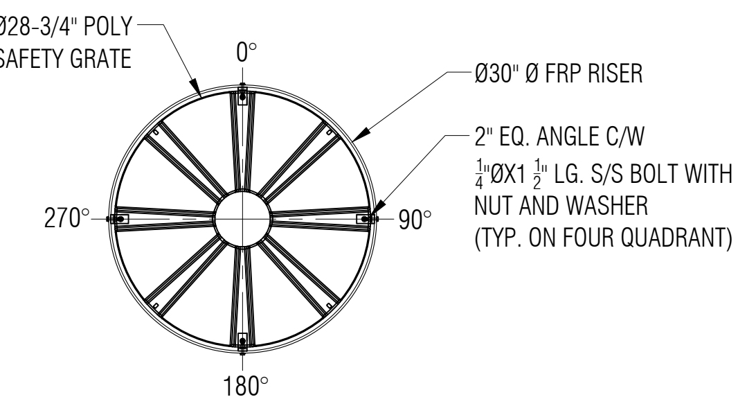
SAFETY GRATE DETAIL G SCALE: 1:15
