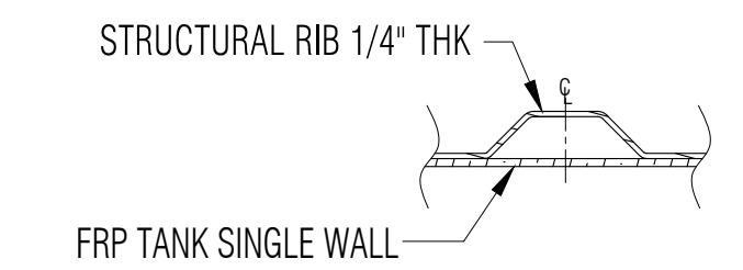
RIB LAMINATE DETAIL F NTS
